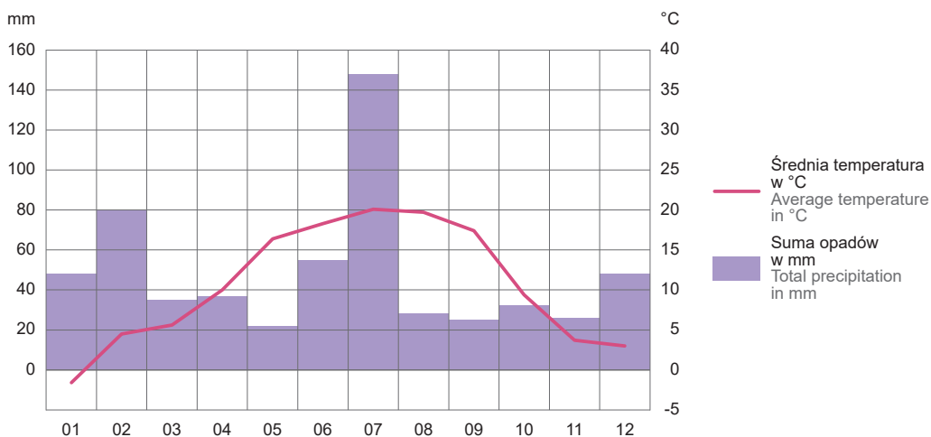
CHART 1. AIR TEMPERATURES AND ATMOSPHERIC PRECIPITATION IN METEOROLOGICAL STATION IN OLSZTYN IN 2024
